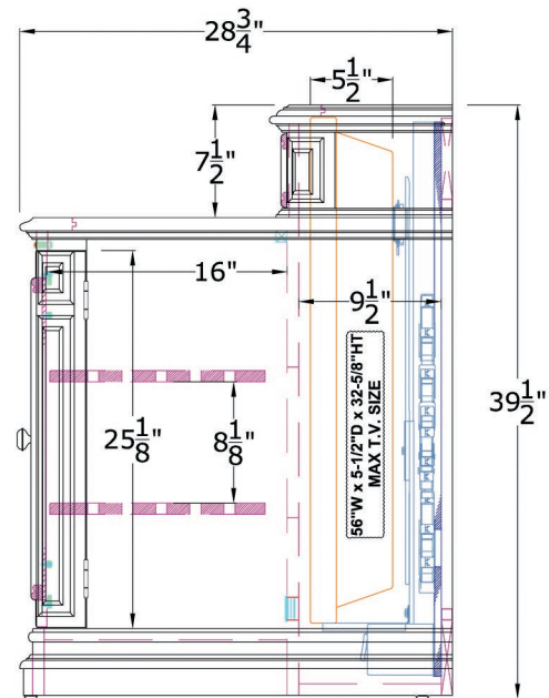
SIDE VIEW (SECTION)
