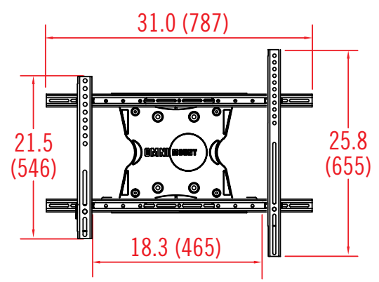
Universal adapter dimensions
